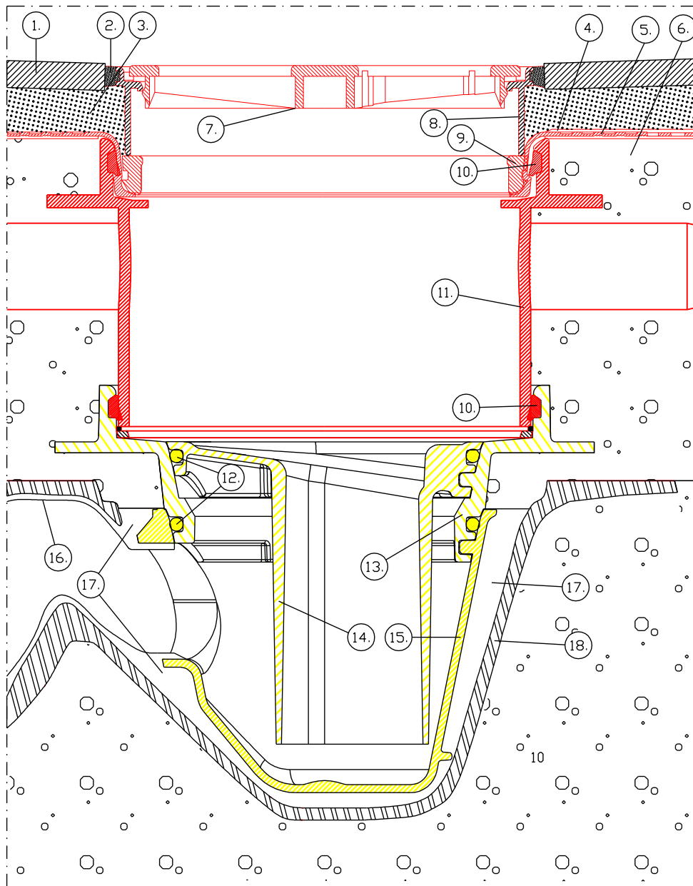
PRINCIPLE SKETCH 1: 2
